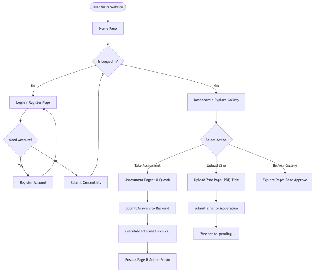
Gambar 3.1 Flowchart Sistem Zine
