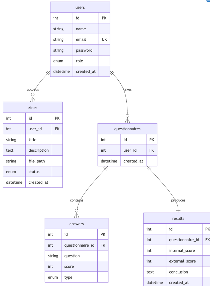
Gambar 3.2 Entity Relationship Diagram (ERD) Sistem Zine
